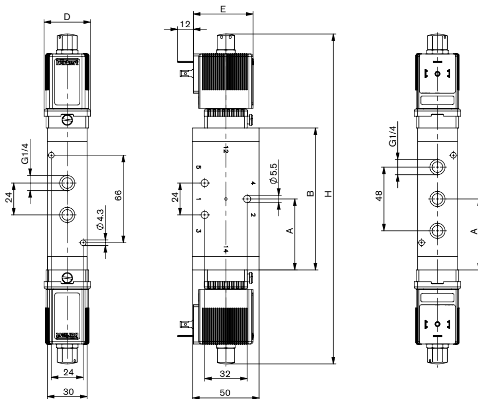
Threaded port version WWH – Impulse, WWL, WWN
